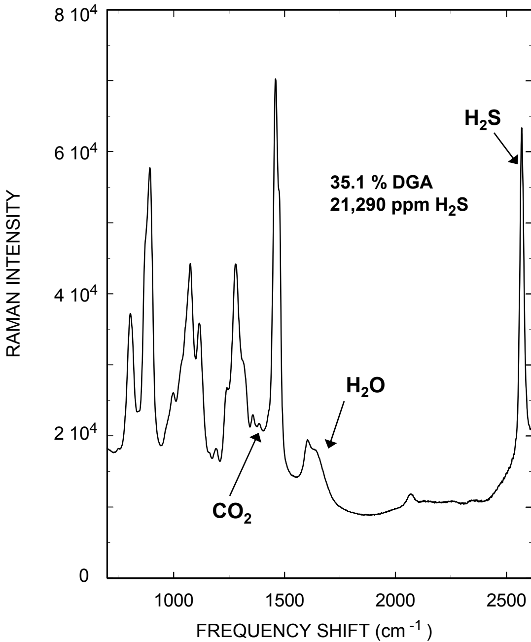
Raman spectrum of Diglycolamine (DGA). Sample contained 35.1 % DGA and 21,290 ppm H 2 S.
